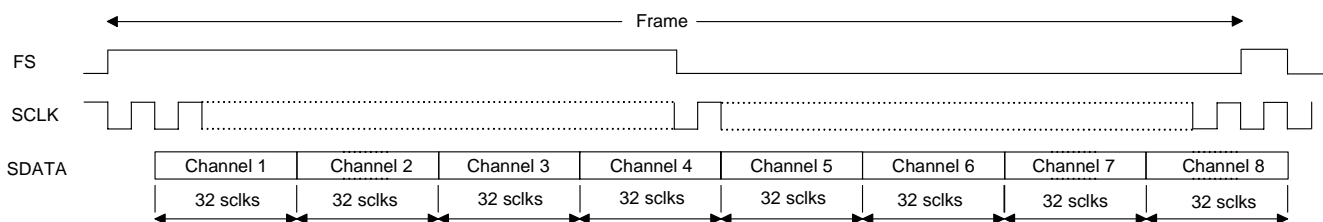
Figure 3. CS5368/66/64 TDM Mode as System Clock Master
