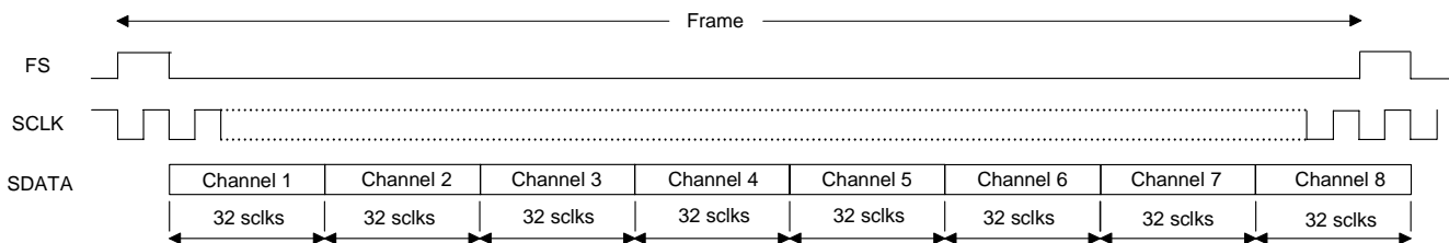
Figure 1. CS4364/65/84/85 TDM Clocking Requirements
