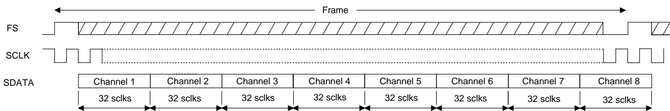
Figure 2. CS5368/66/64 TDM Mode as System Clock Slave
