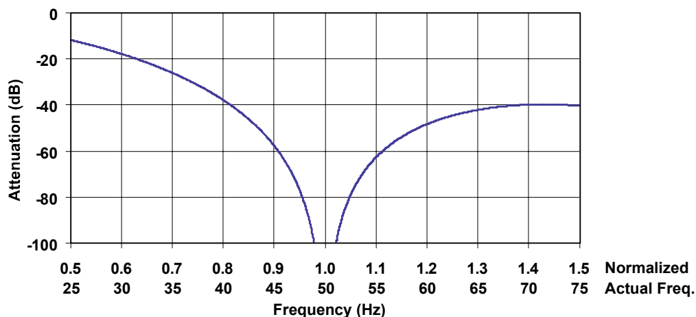
Figure 3. Third-order Sinc Filter Response (Sinc 3 ), Normalized to 1
