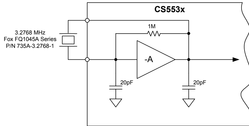
Figure 5. CS5530/31/32/33/34 Crystal Oscillator Circuit
