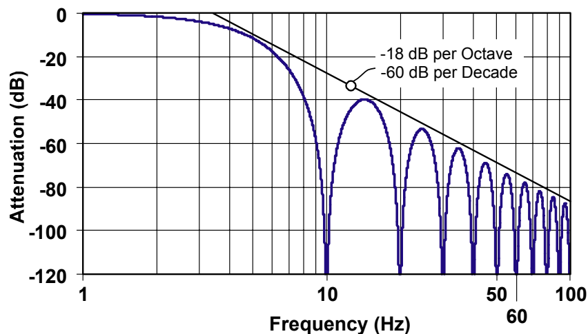
Figure 4. Third-order Sinc Filter Response (Sinc 3 )
