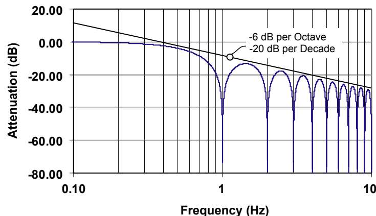
Figure 1. First-order Sinc ( \text{Sinc}^1 ) Filter Response
