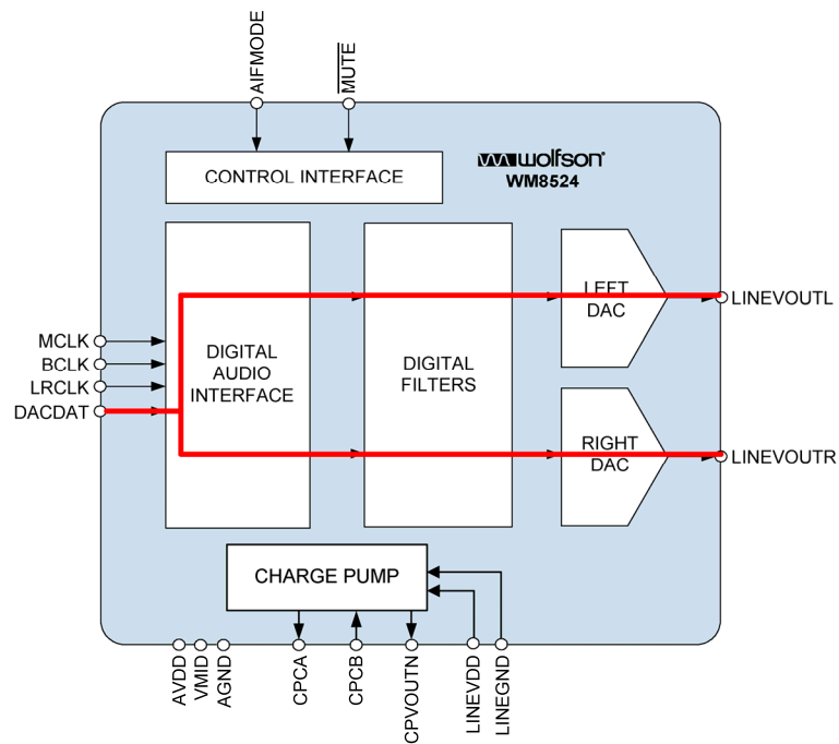
Figure 2 DAC Playback to Line Out
