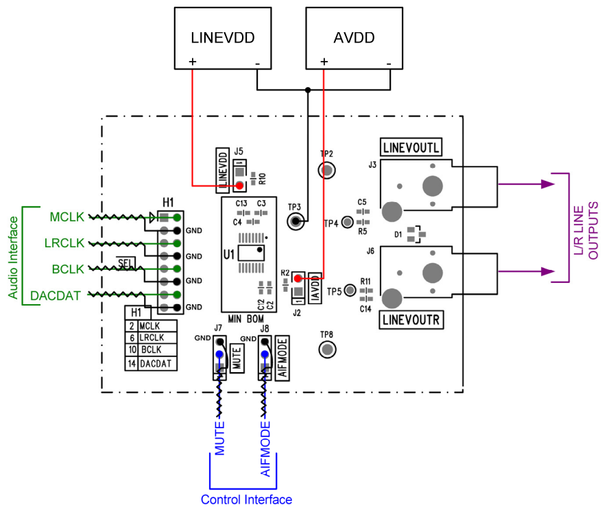
Figure 1 Stand-Alone Board Configuration
