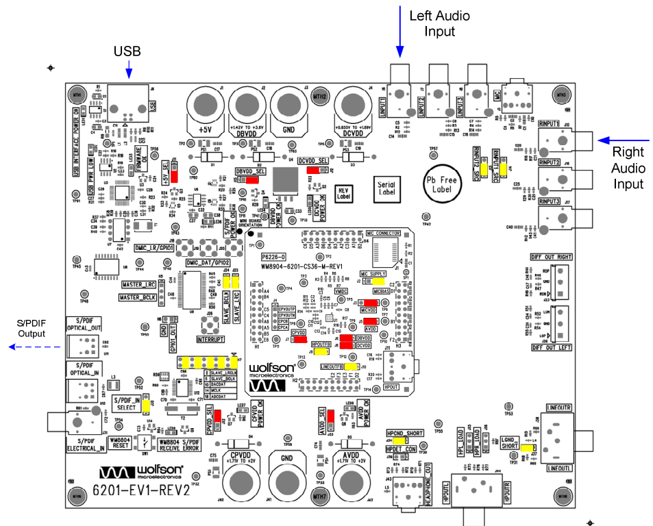
Figure 6 Board Configuration IN1L/R to ADC
