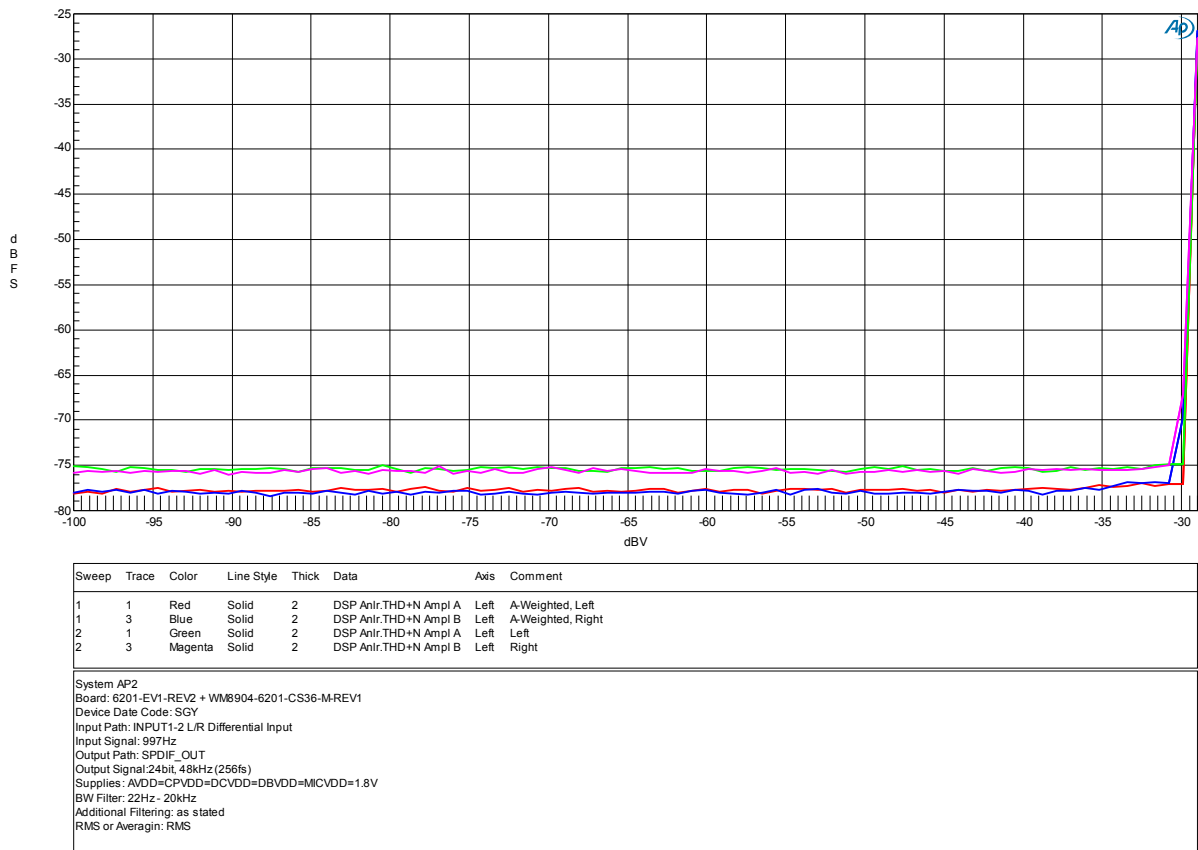
Figure 10 Performance Plot IN1L+2L / IN1R+2R to ADC (differential MIC)
