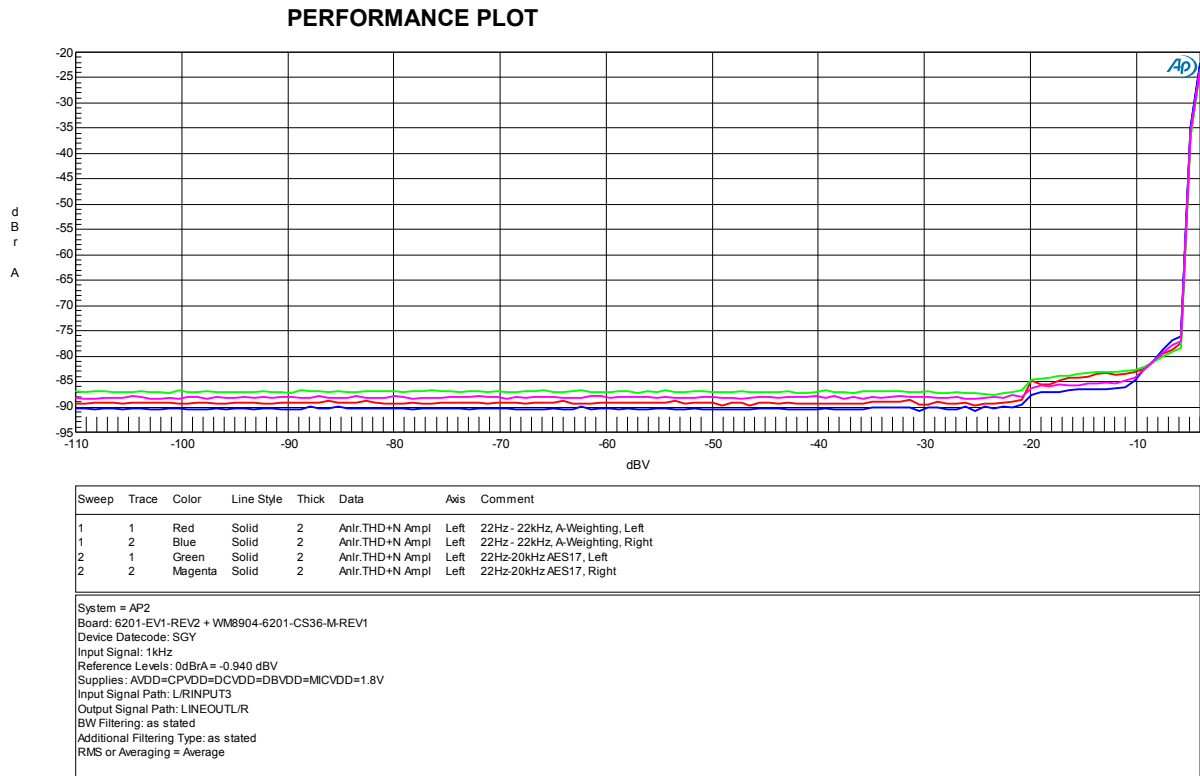
Figure 15 Performance Plot IN3L/R to LINEOUTL/R (digital loopback)
