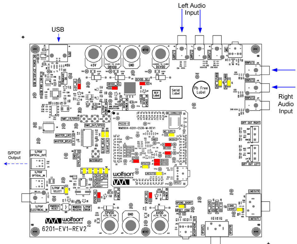
Figure 9 Board Configuration IN1L+2L / IN1R+2R to ADC
