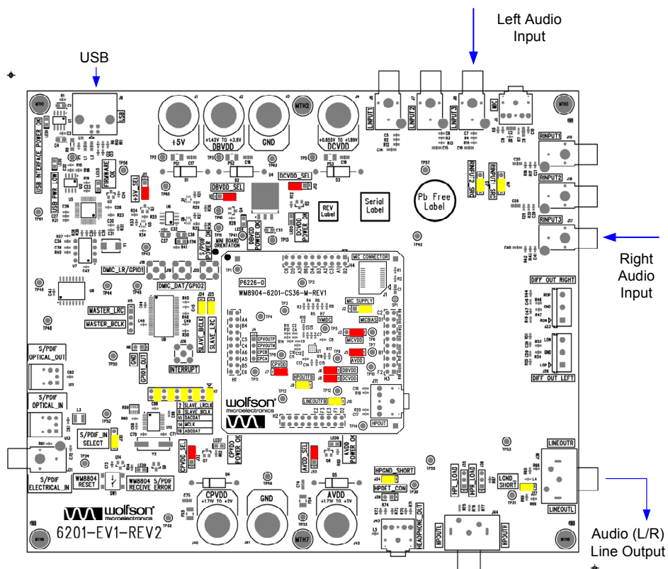
Figure 12 Board Configuration IN3L/R to LINEOUTL/R
