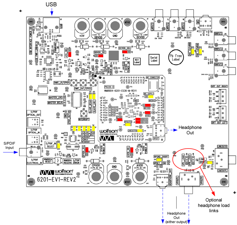
Figure 3 Board Configuration DAC to HPOUTL/R
