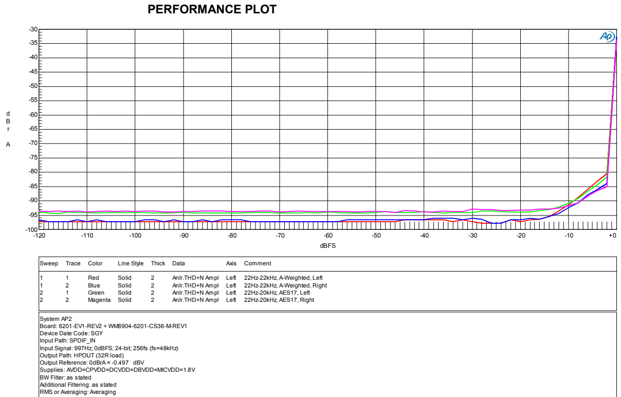
Figure 4 Performance Plot DAC to HPOUTL/R
