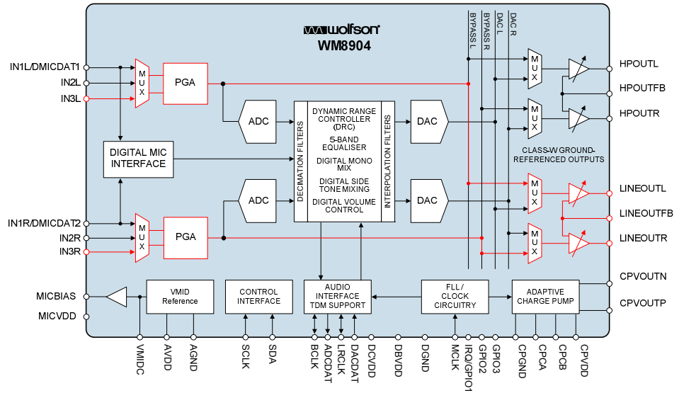
Figure 11 Path Diagram IN3L/R to LINEOUTL/R
