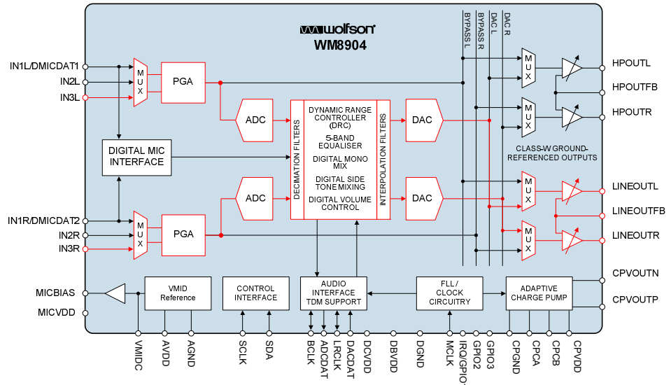
Figure 14 Path Diagram IN3L/R to LINEOUTL/R (digital loopback)
