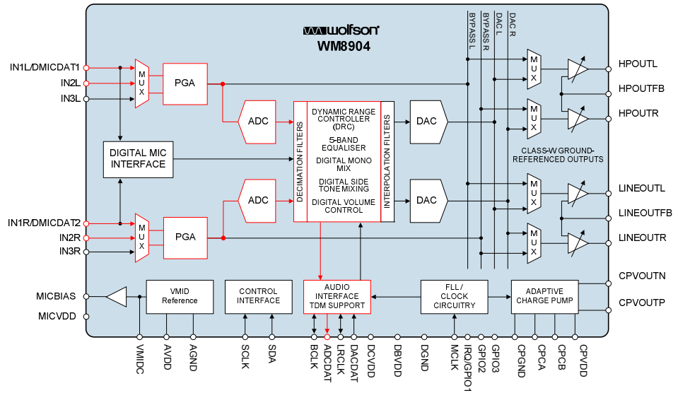
Figure 8 Path Path Diagram IN1L+2L / IN1R+2R to ADC
