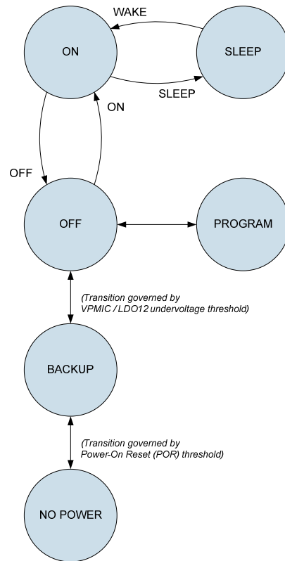
Figure 1 Power States and Transitions
