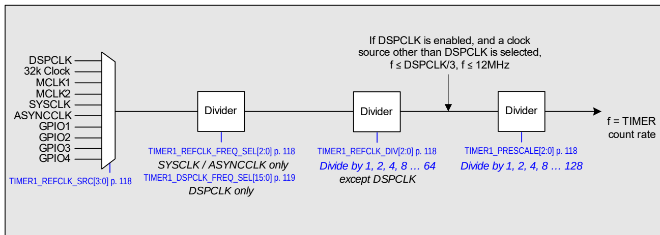
Figure 4-35. General-Purpose Timer
