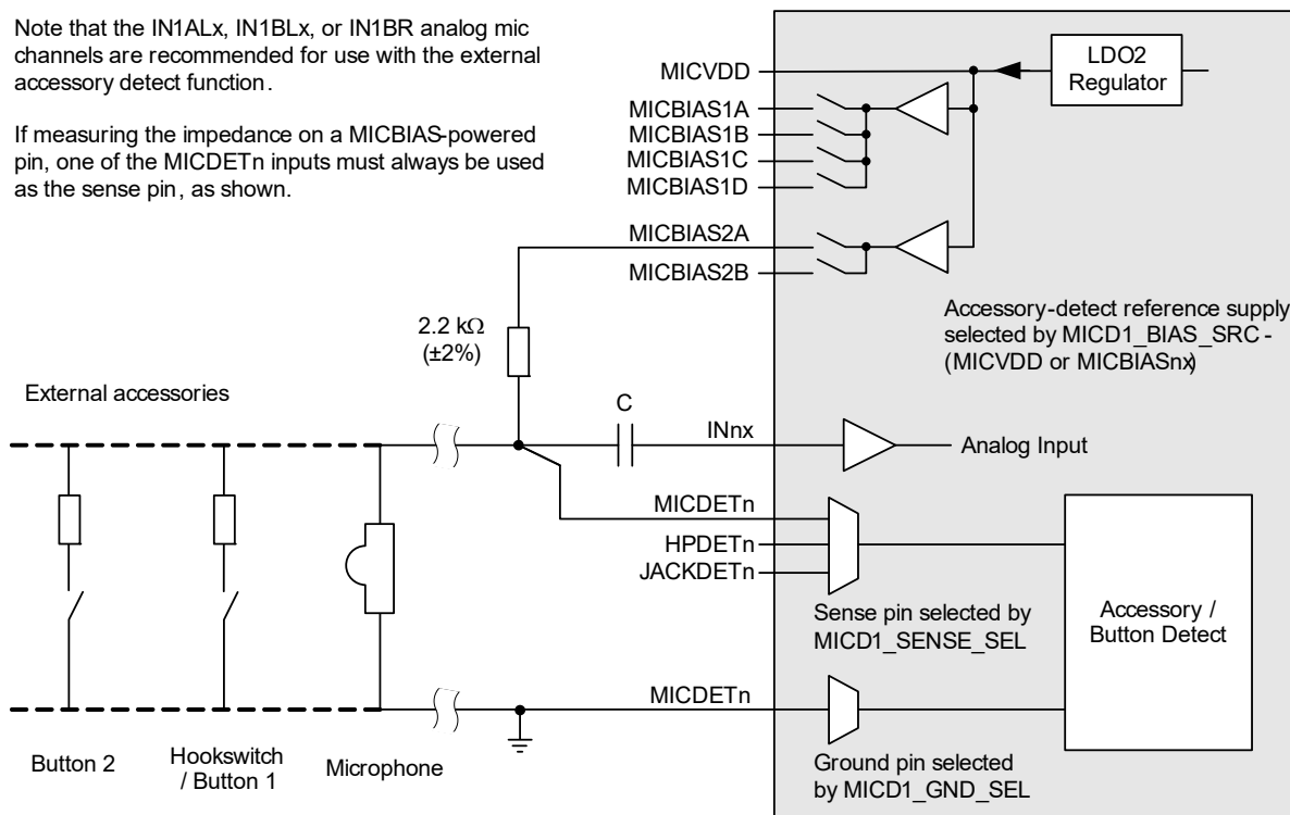
Figure 4-61. Microphone- and Accessory-Detect Interface
