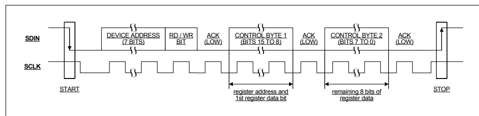
Figure 26 2-Wire Serial Control Interface
