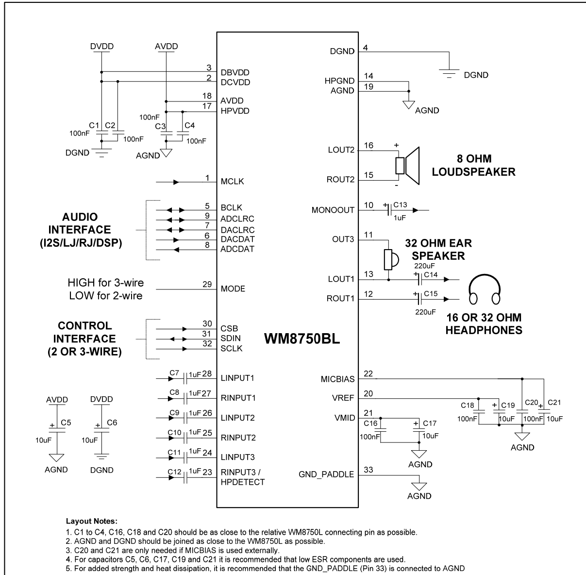
Figure 50 Recommended External Components Diagram
